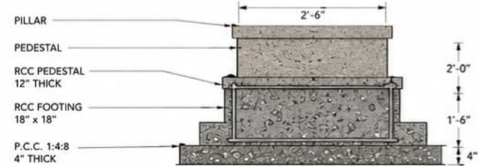
FOUNDATION DETAIL
