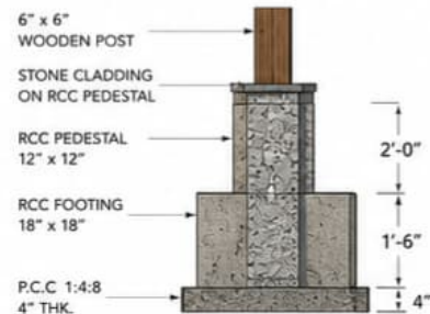
FOUNDATION DETAIL
