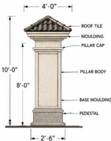
SIDE ELEVATION (LEFT VIEW)
