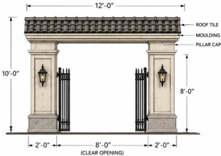
ELEVATION (FRONT VIEW)
