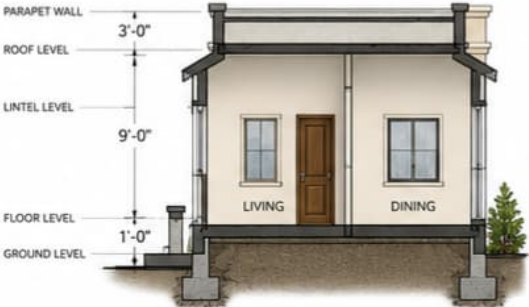
BUILDING SECTION (A-A)
